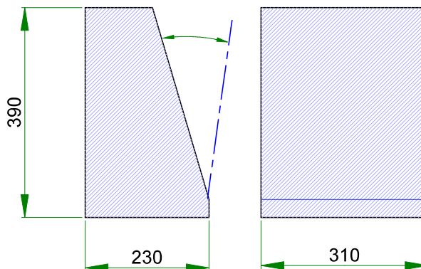
Overall dimensions.
